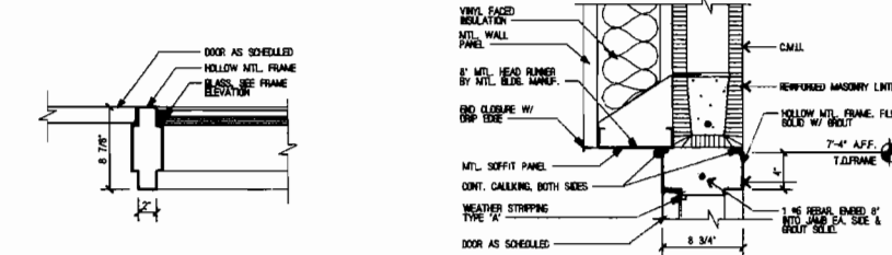
3 DOOR-WINDOW MULLION SCALE: 1 1/2"=1'-0" HMD/HME
