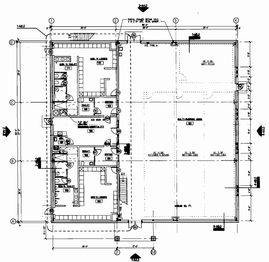
1 FIRST FLOOR PLAN SCALE: 1/8"=1'-0"
