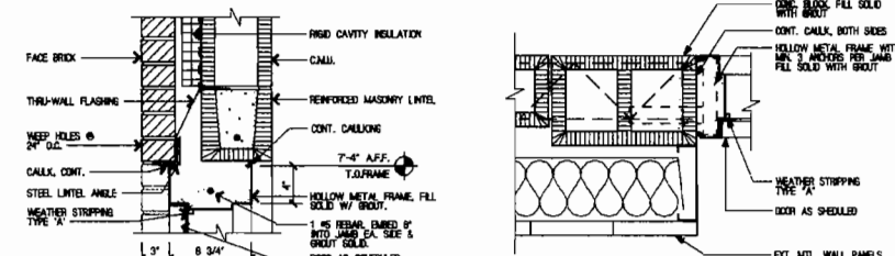
4 DOOR HEAD SCALE: 1 1/2"=1'-0" HMB/HMC
