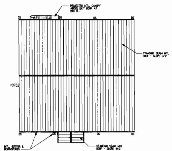
3 ROOF PLAN SCALE: 1/8"=1'-0"
