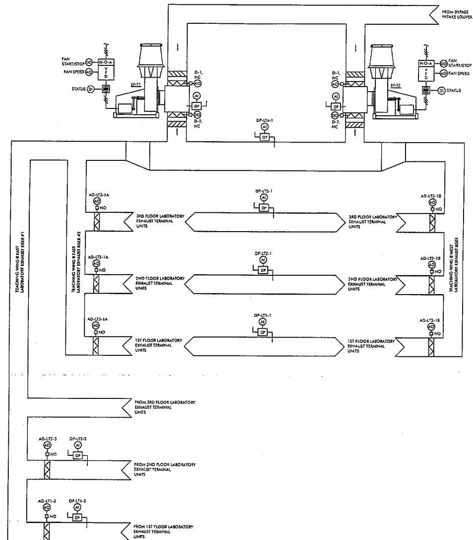
1 CONTROL DIAGRAM - TEACHING WING B LABORATORY EXHAUST SYSTEM SCALE: NONE
