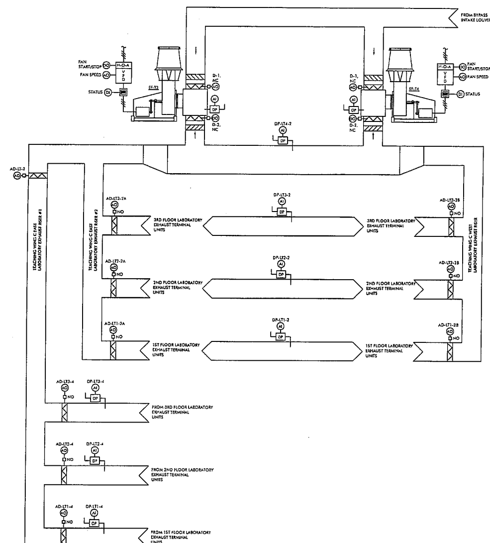
2 CONTROL DIAGRAM - TEACHING WING C LABORATORY EXHAUST SYSTEM SCALE: NONE
