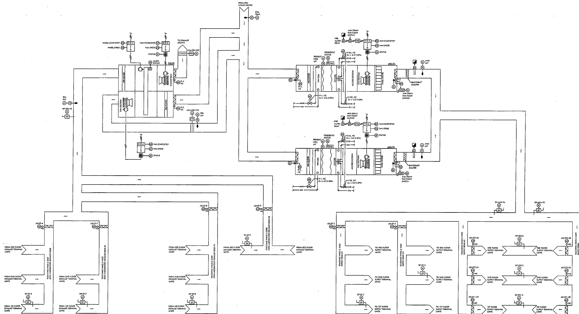
1 CONTROL DIAGRAM - TEACHING WING C SUPPLY AIR & NON-LABORATORY EXHAUST SYSTEM M&9 SCALE: NONE
