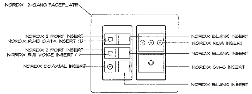
FACEPLATE "A" TEACHER MULTIMEDIA LOCATION
