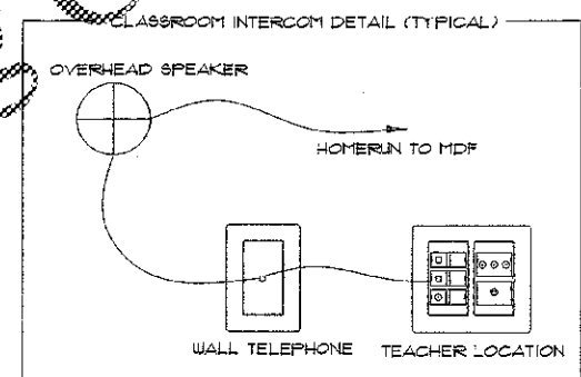
CLASSROOM INTERCOM DETAIL (TYPICAL)
