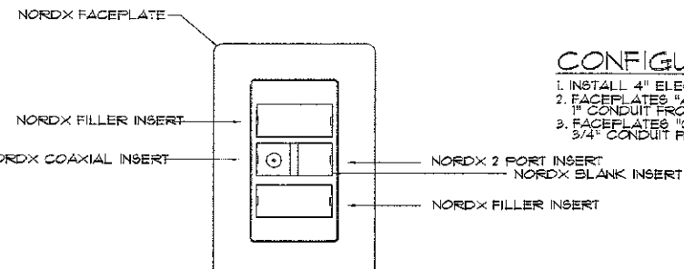
FACEPLATE "H" STANDARD TV OUTLET
