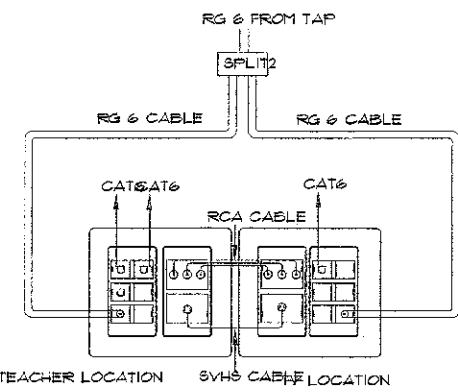
TEACHER/TV DETAIL
