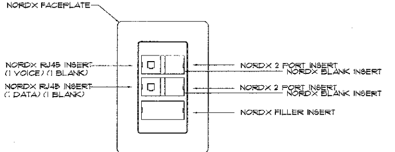
FACEPLATE "G" VOICE/DATA LOCATION
