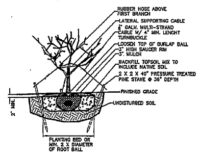
MULTIPLE TRUCK TREE DETAIL NOT TO SCALE
