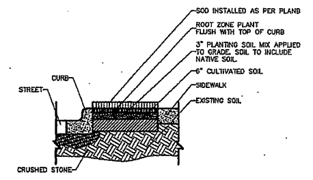
SOD PLACEMENT DETAIL NOT TO SCALE
