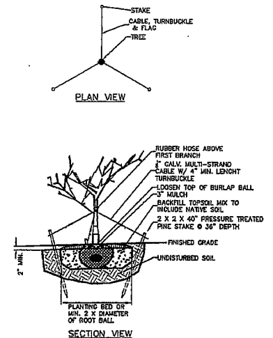
TREE PLANTING DETAIL NOT TO SCALE
