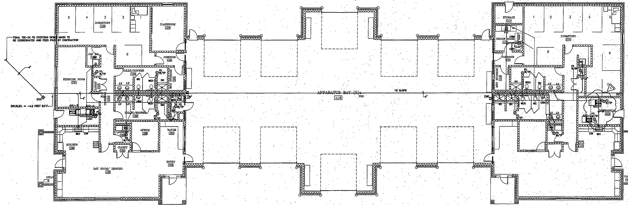
FLOOR PLAN PLUMBING-GRAVITY NORTH 0 2 4 6 8 16 SCALE: 1/8" = 1'-0"
