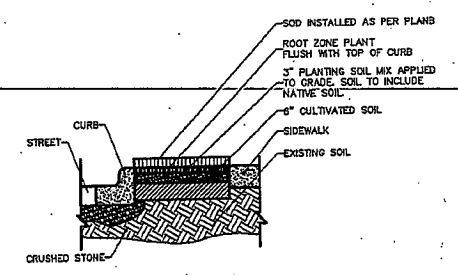
SOD PLACEMENT DETAIL NOT TO SCALE
