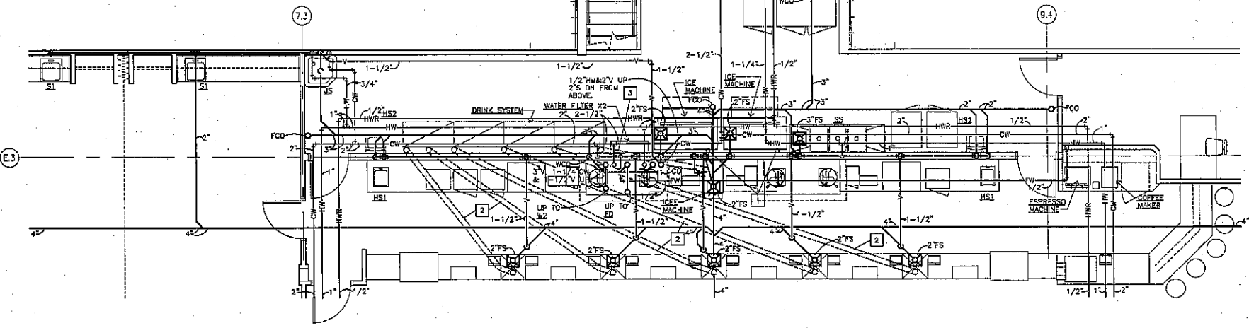
PARTIAL FLOOR PLAN - PLUMBING 1/4" = 1'-0"
