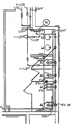
PARTIAL FLOOR PLAN - PLUMBING 1/4" = 1'-0"
