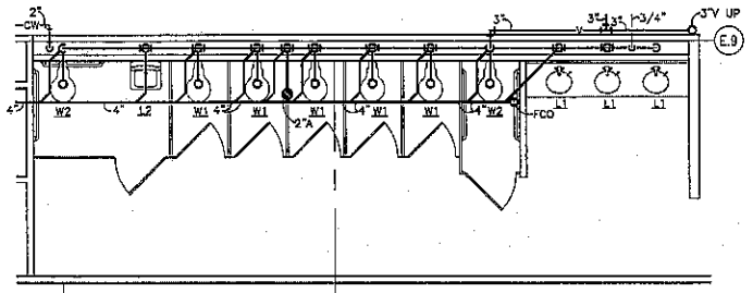
PARTIAL FLOOR PLAN - PLUMBING 1/4" = 1'-0"
