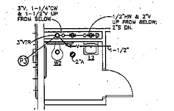
PARTIAL MEZZANINE FLOOR PLAN - PLUMBING 1/4" = 1'-0"
