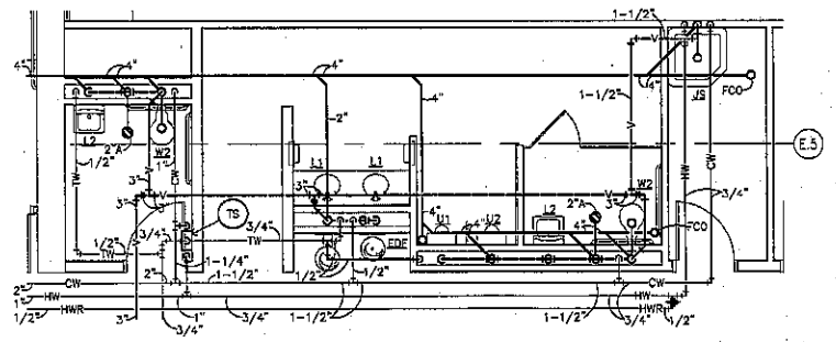
PARTIAL FLOOR PLAN - PLUMBING 1/4" = 1'-0"
