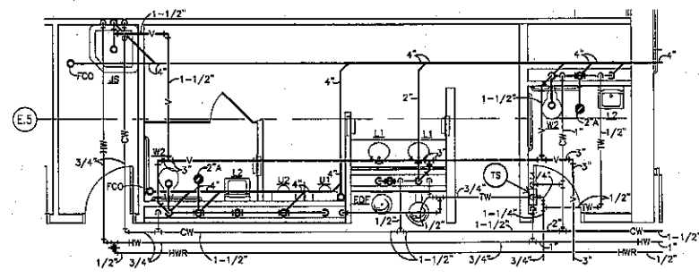
PARTIAL FLOOR PLAN - PLUMBING 1/4" = 1'-0"
