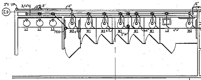
PARTIAL FLOOR PLAN - PLUMBING 1/4" = 1'-0"
