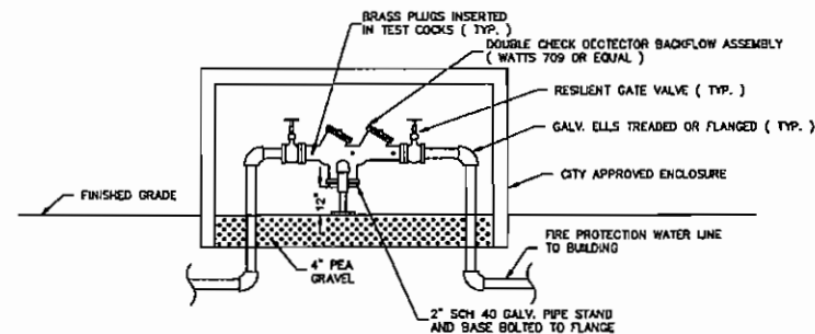
6" DOUBLE CHECK DETECTOR VALVE BACKFLOW PREVENTOR N.T.S.
