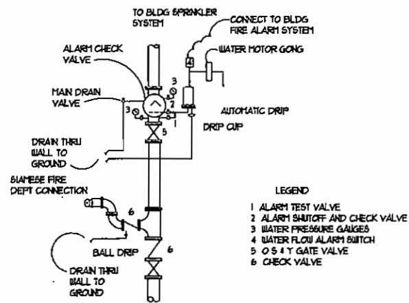
SPRINKLER RISER DETAIL SCHEMATIC ONLY
