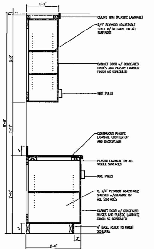
REF: A701 11 MILLWORK SECTION SCALE: 1" = 1'-0"
