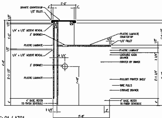
REF: 01 / A701 03 MILLWORK SECTION
