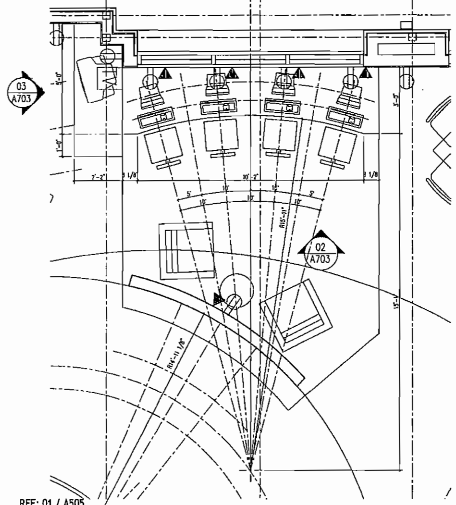
REF: 01 / A505 01 MILLWORK ELEVATION SCALE: 1/2" = 1'-0"
