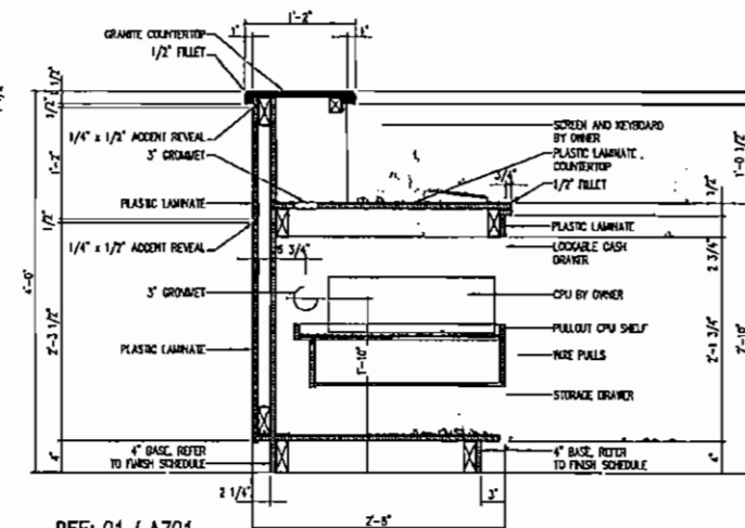
REF: 01 / A701 02 MILLWORK SECTION
