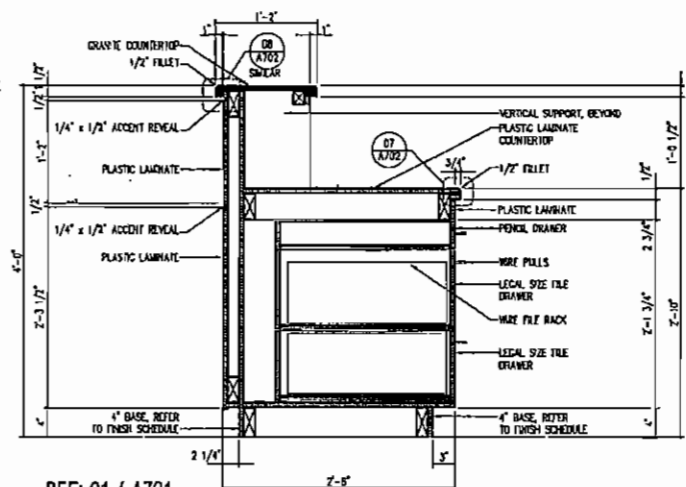
REF: 01 / A701 01 MILLWORK SECTION
