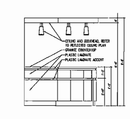
REF: 01 / A701 03 MILLWORK ELEVATION
