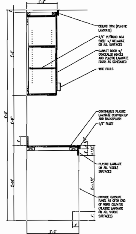
REF: 06/A701, 08/A701 12 MILLWORK SECTION SCALE: 1" = 1'-0"
