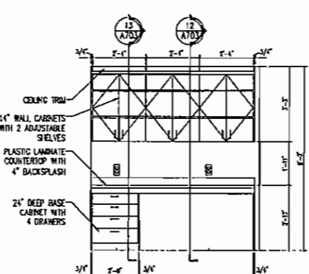
REF: A501 06 MILLWORK ELEVATION SCALE: 3/8" = 1'-0"
