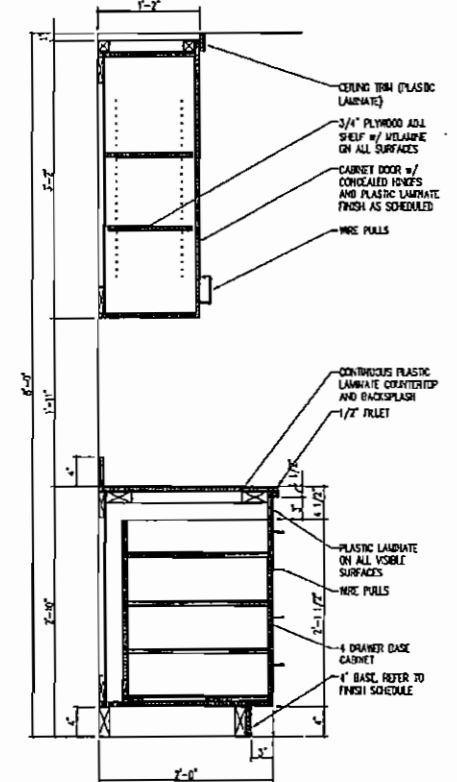
REF: 06/A701, 08/A701 13 MILLWORK SECTION SCALE: 1" = 1'-0"
