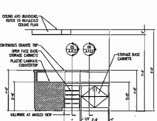
REF: 01 / A701 05 MILLWORK ELEVATION SCALE: 3/8" = 1'-0"
