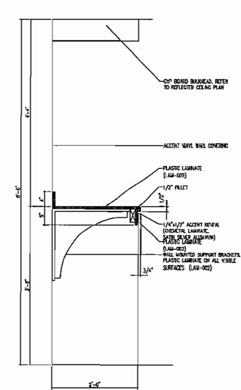
REF: A701 12 MILLWORK SECTION SCALE: 1" = 1'-0"
