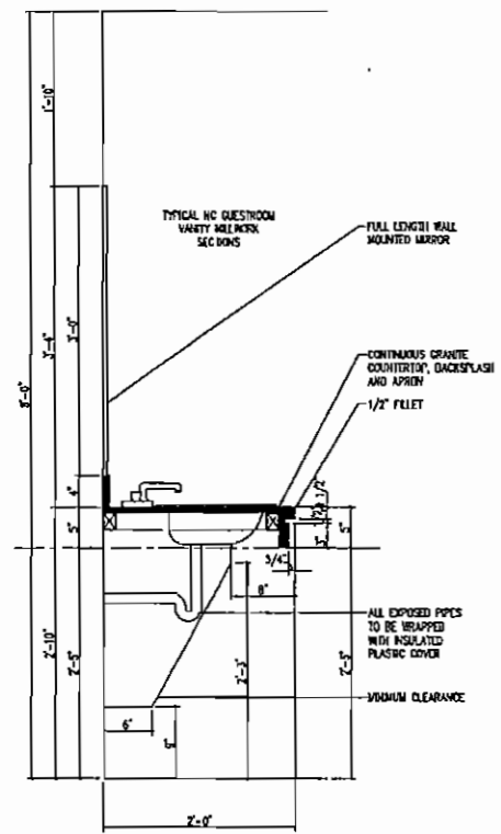
REF: 10/A507, 10/A509 15 MILLWORK SECTION SCALE: 1" = 1'-0"
