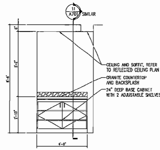
REF: A501 13 MILLWORK ELEVATION SCALE: 1/2" = 1'-0"
