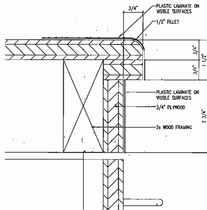
REF: 01 / A702 07 MILLWORK DETAIL
