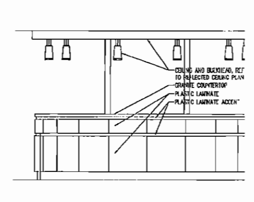
REF: 01 / A701 02 MILLWORK ELEVATION SCALE: 3/8" = 1'-0"
