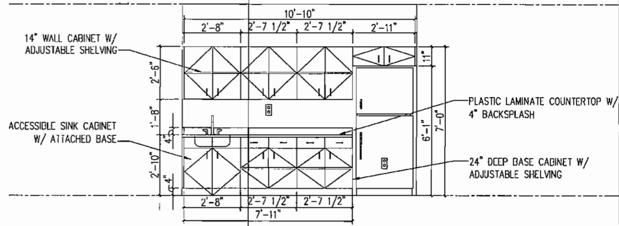
REF: 01 / A701 04 MILLWORK ELEVATION
