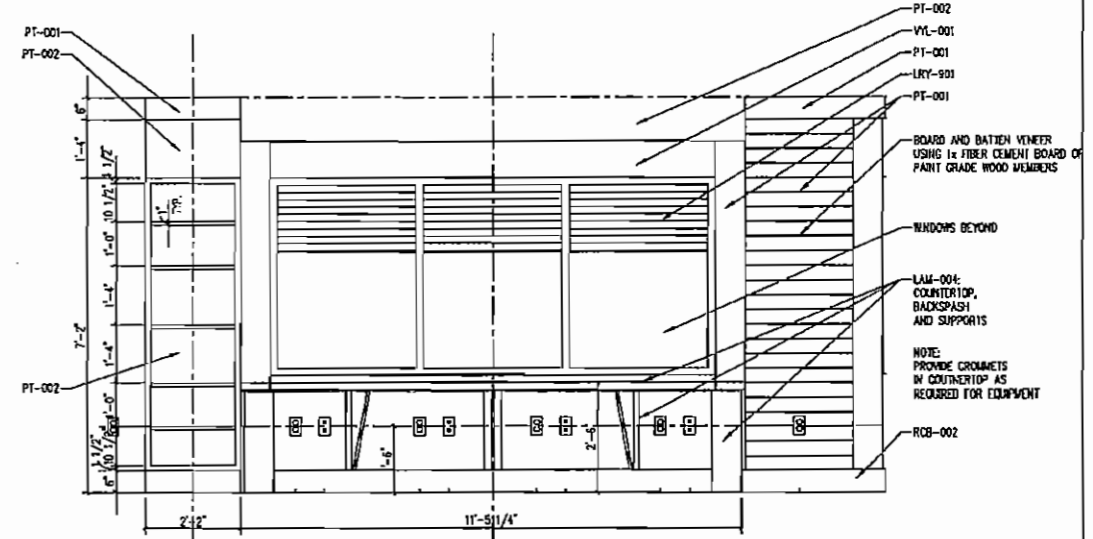
REF: 01 / A505 02 MILLWORK ELEVATION SCALE: 1/2" = 1'-0"
