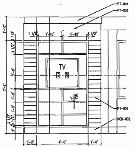
REF: 01 / A505 03 MILLWORK ELEVATION SCALE: 1/2" = 1'-0"
