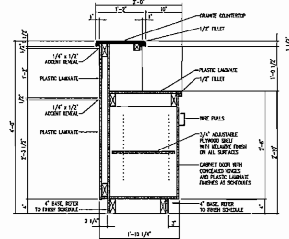
REF: 01 / A701 06 MILLWORK SECTION
