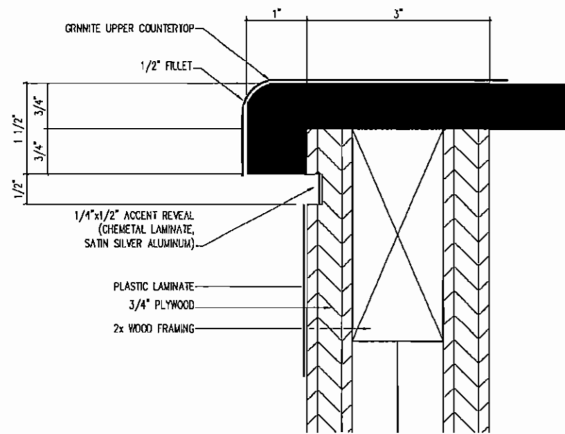
REF: 01 / A702 08 MILLWORK DETAIL
