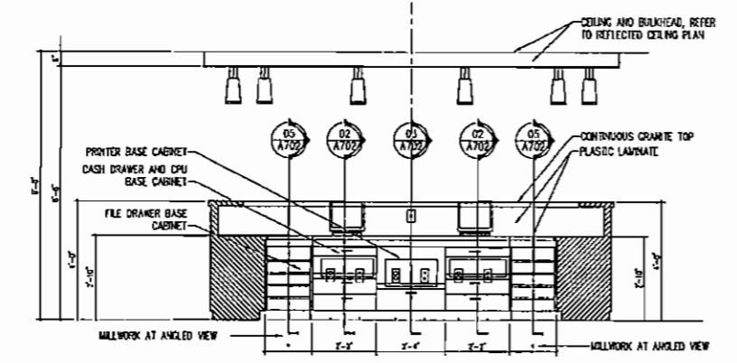
REF: 01 / A701 04 MILLWORK ELEVATION SCALE: 3/8" = 1'-0"
