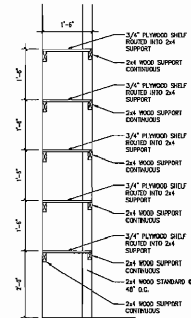
09 STORAGE SHELVING SECTION
