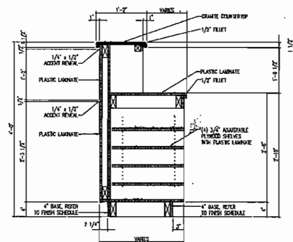
REF: 01 / A701 05 MILLWORK SECTION
