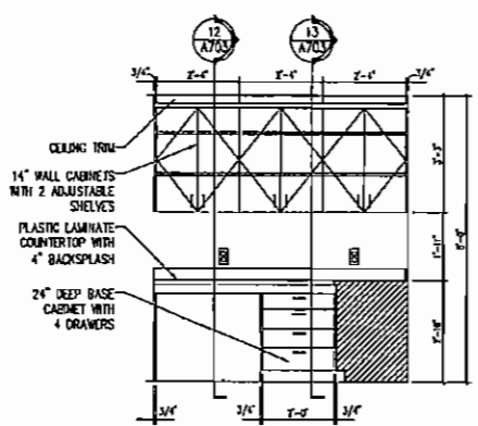
REF: A501 08 MILLWORK ELEVATION SCALE: 3/8" = 1'-0"
