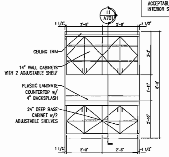
REF: A501 09 MILLWORK ELEVATION SCALE: 1/2" = 1'-0"
